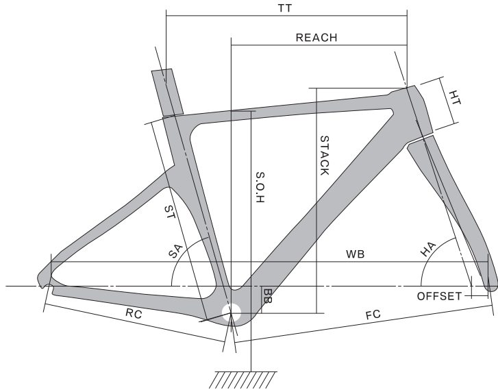
EDGE700 Carbon Frame Original Geometry Size Chart
