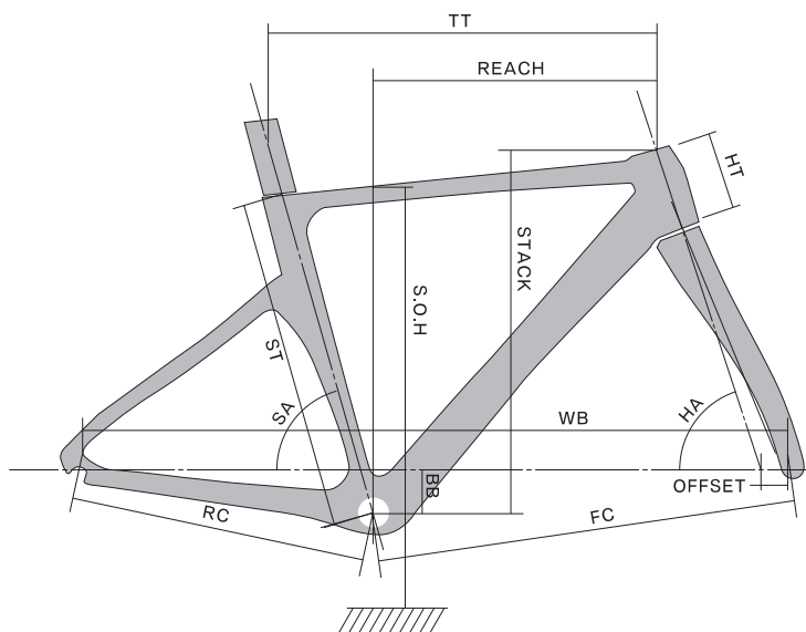
EDGE700D Carbon Frame Original Geometry Size Chart
